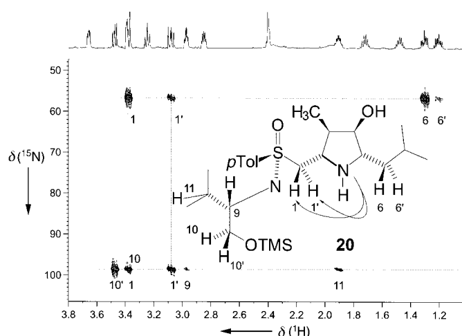
Figure 2. Part of the 15 N– 1 H HMBC spectrum of 20 . Verification of the cyclization (thick bond) is provided by the correlation of the pyrrolidine nitrogen atom to the protons (1, 1') of the sulfonimidomethyl group.
