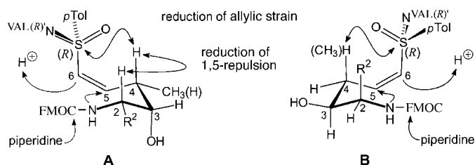
Figure 1. Stereochemical aspects of the cyclization. The topicity of the attack of the nitrogen atom on the 5-position is directed by two conformational aspects: reduction of allylic strain and 1,5-repulsion.
