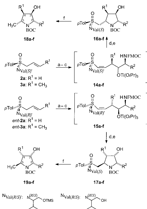
Scheme 2. Synthesis of pyrrolidines 18a–f and 19a–f , starting from open-chain 2-alkenylsulfoximides. a) n BuLi, –78 °C. b) Chlorotris(isopropoxy)-titanium, 0 °C. c) 21a–c , –78 °C. d) Piperidine, 20 °C; (NH 4 ) 2 CO 3 , NH 4 Cl. e) K 2 CO 3 , MeOH; BOC 2 O, NaHCO 3 . f) SmI 2 . Fmoc = (9H-fluoren-9-ylmethoxy)carbonyl.
