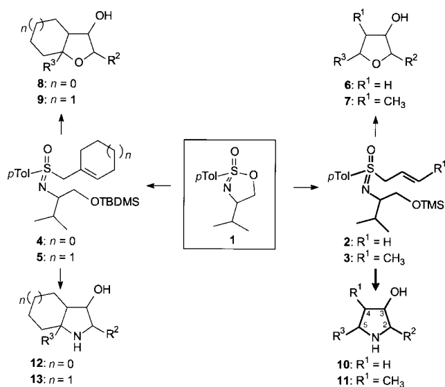
Scheme 1. Heterocyclic compounds available from the cyclic sulfonimide 1 . R 2 = alkyl, alkaryl, alkheteroaryl; R 3 = CH 2 S(O)(pTol)N val , vinyl, methyl. TMS = trimethylsilyl, TBDMS = tert -butyldimethylsilyl.
